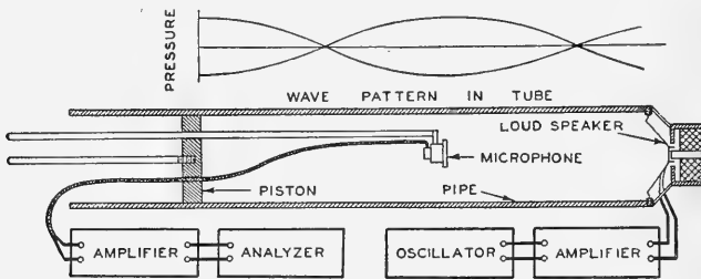
FIG. 11.4. Arrangement of apparatus for measuring the non-linear distortion generated by a microphone. (After Phelps.)
